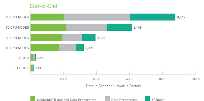
Fig.3: Performance testing: CPU vs. GPU-accelerated ML workflow
